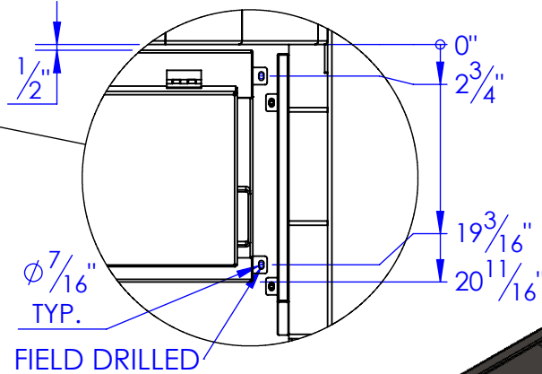
DETAIL B SCALE 1 : 15
